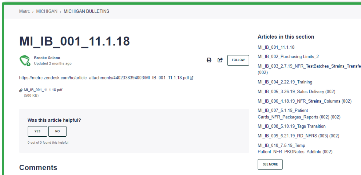
Figure 8: Bulletin Page
