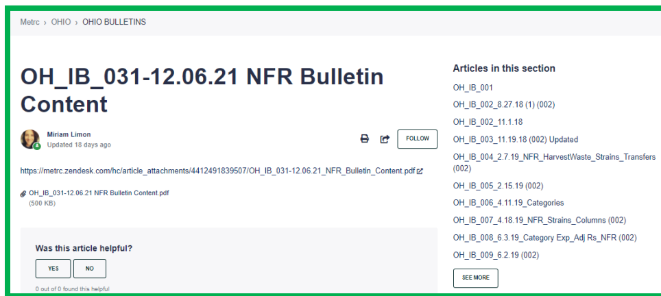
Figure 8: Bulletin Page
