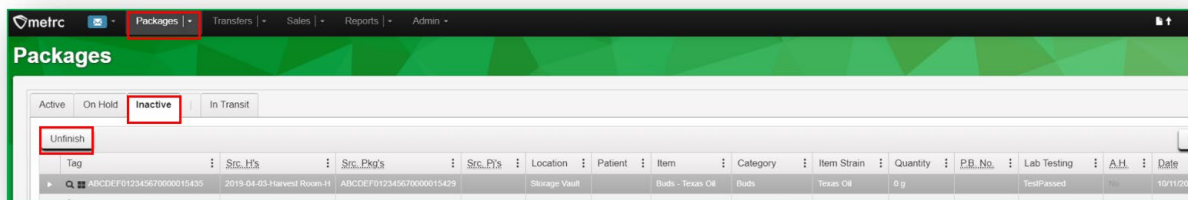
Figure 7: Unfinishing Packages
