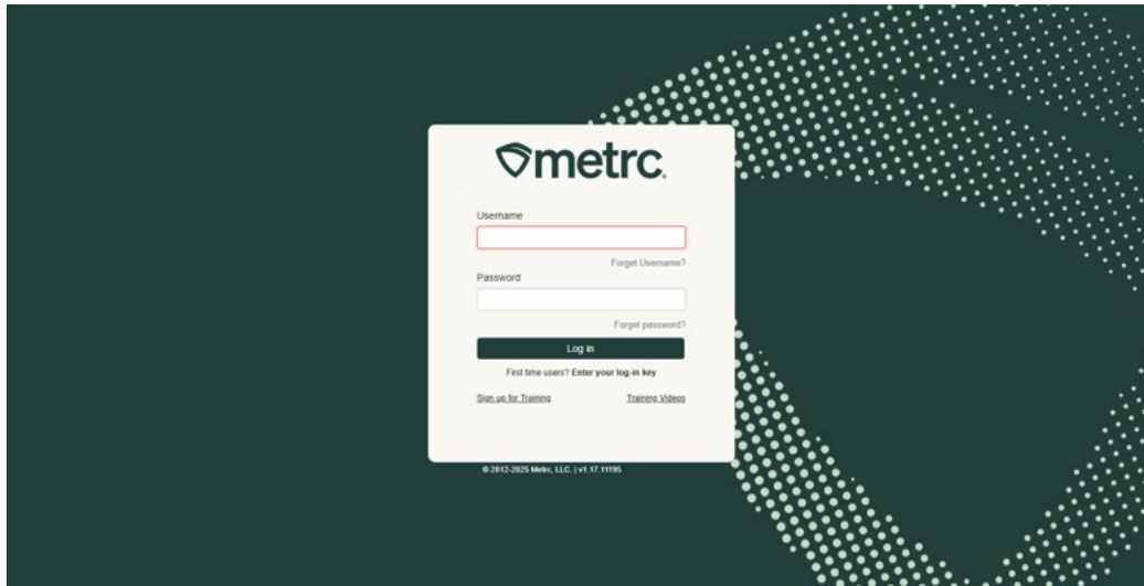
Figure 2 - Login screen
